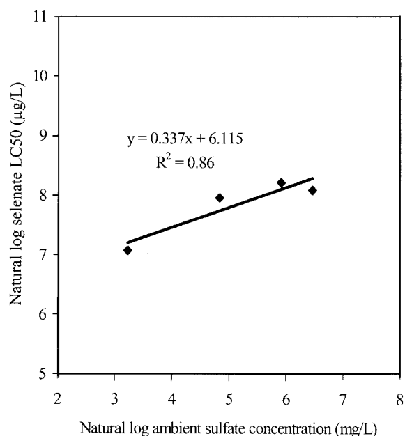
Fig. 4. Relationship between ambient sulfate concentration and acute selenate toxicity for Gammarus pseudolimnaeus .
